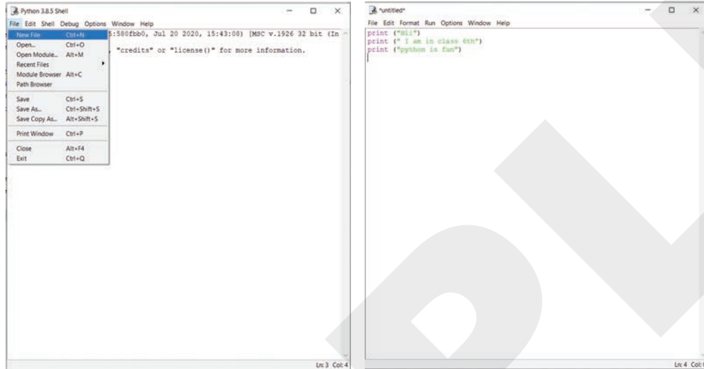
Figure 6.9 Screenshots 2 & 3
