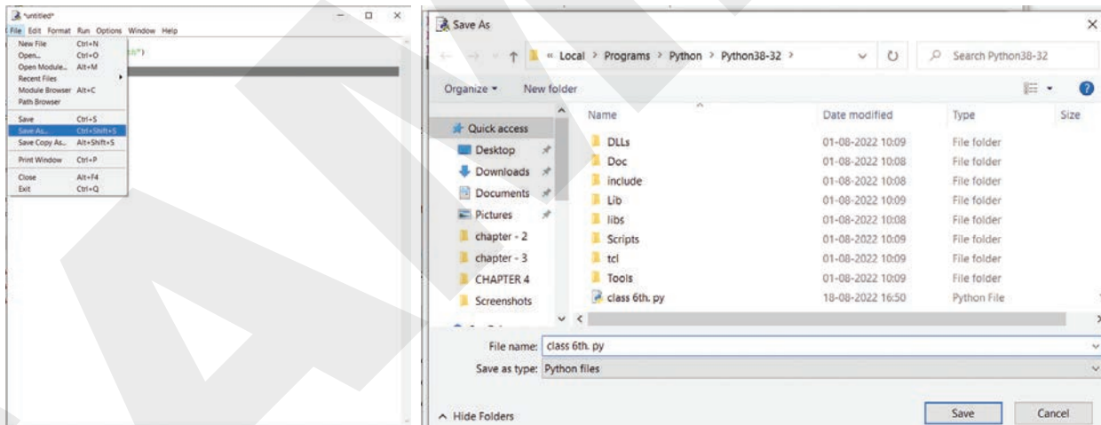
Figure 6.10 Screenshots 4 & 5
