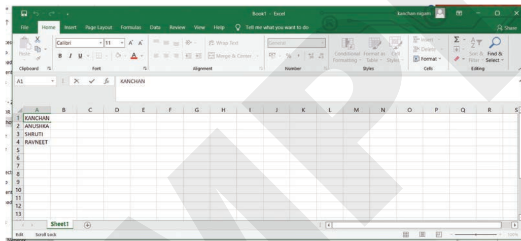
Figure 3.4 Edit Mode.
