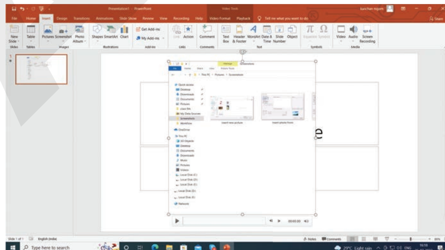
Figure 2.6 Inserting Screenshot
