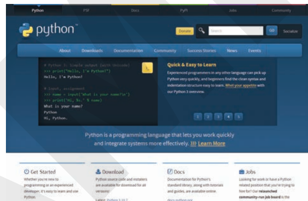
Figure 6.1 Installing Python
