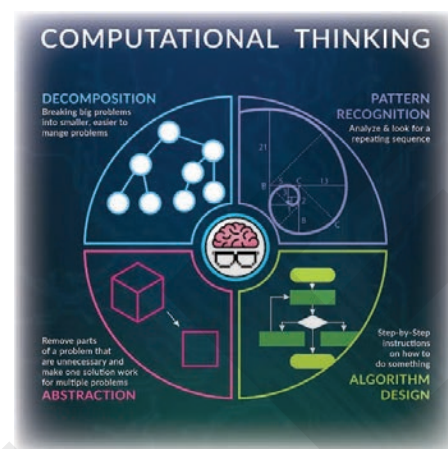
Figure 5.1 Computational Thinking
