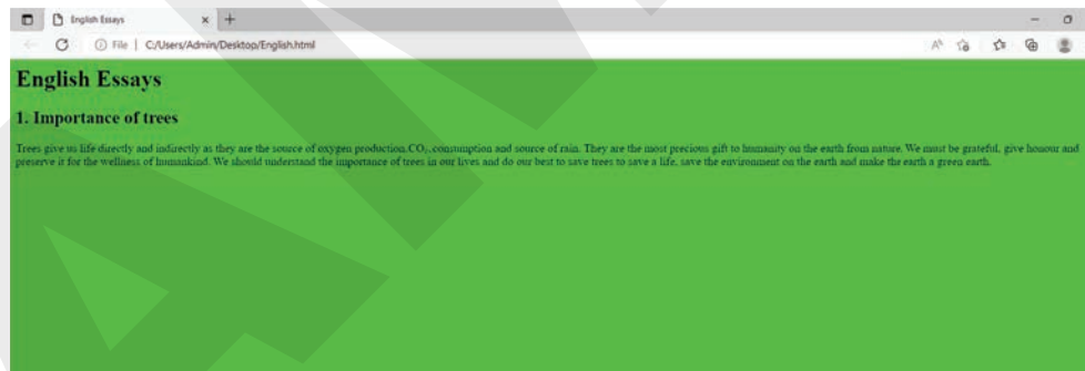
Figure 7.1 Web page
