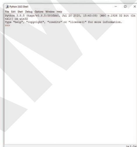
Figure 6.6 Python IDLE
