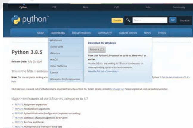
Figure 6.2 Python Download
