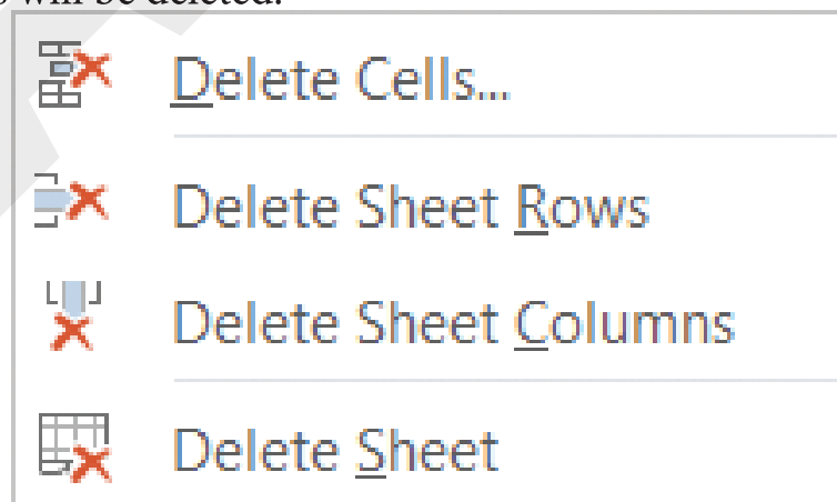
Figure 3.7 Delete Cells
