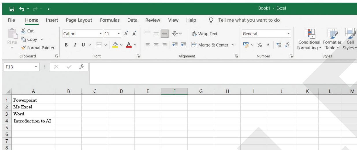
Figure 3.1 Editing Cells
