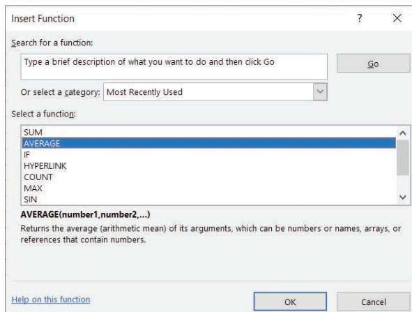
Figure 4.9 Insert Function
