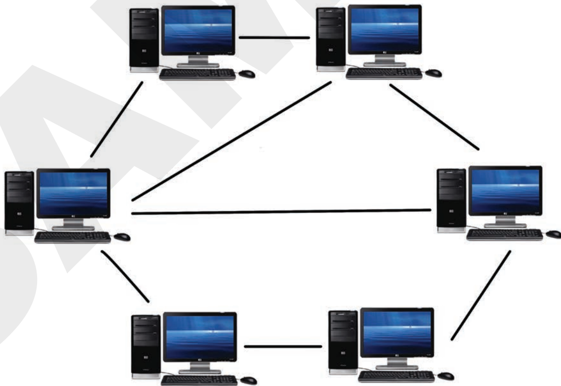
Figure 1.10: Peer-to-Peer Network
