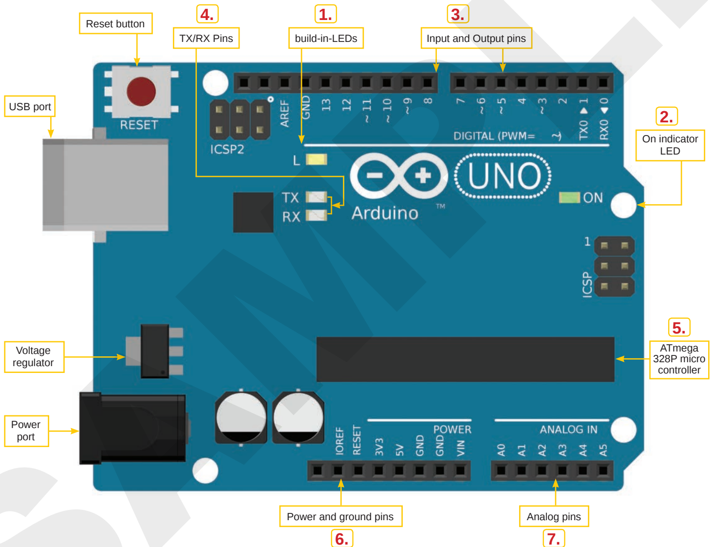
Figure 5.2: Parts of an Arduino Board
