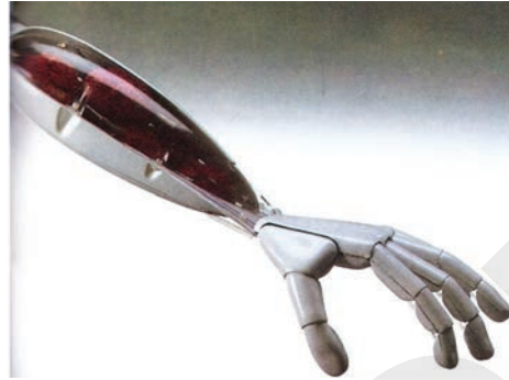
Figure 7.3: Pneumatic Air Muscles
