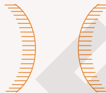
Concave mirror Convex mirror
