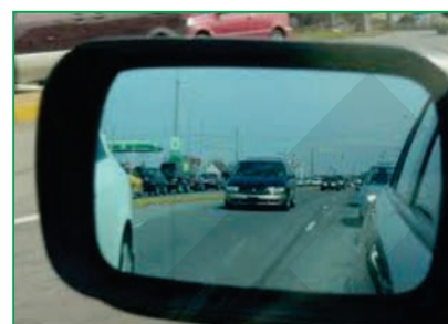
Convex mirror or side view mirror
