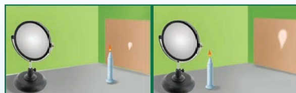
Real images formed by a concave mirror
