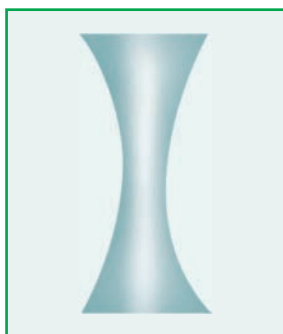
A Concave Lens
