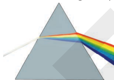
Dispersion
