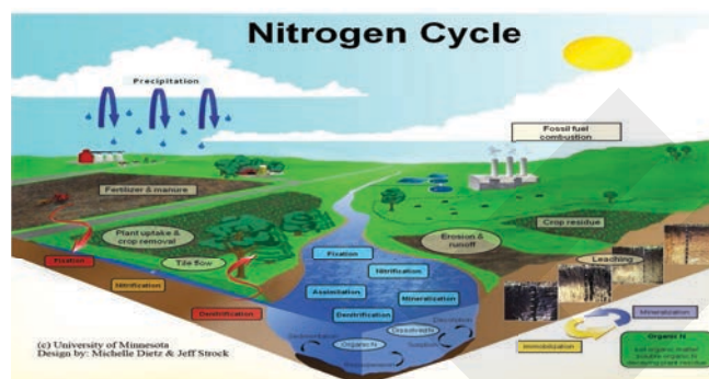
Nitrogen Cycle
