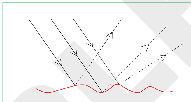
Diffused reflection
