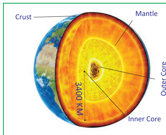
The inner structure of the earth (not to the scale)
