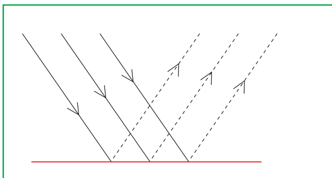
Regular reflection
