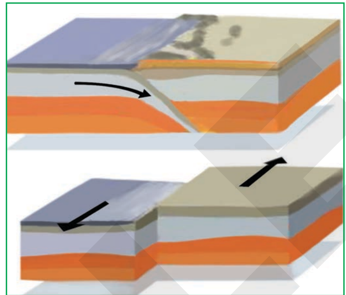
Movements of earth's plates
