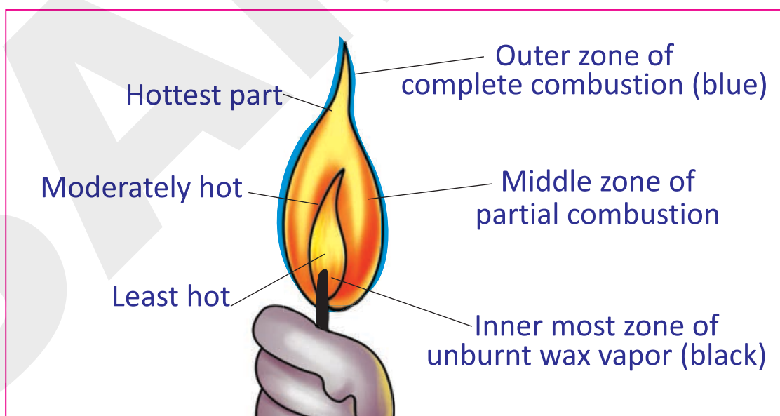
Different zones of a Candle
