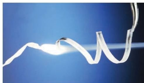
Burning of magnesium ribbon
