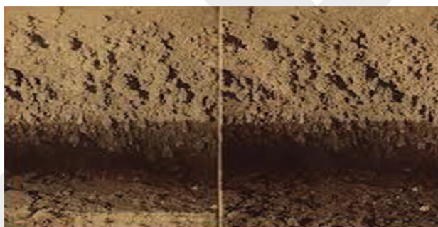
Formation of Coal
